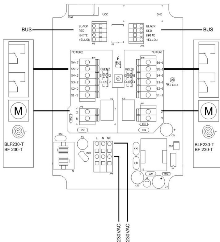
Wiring diagram
